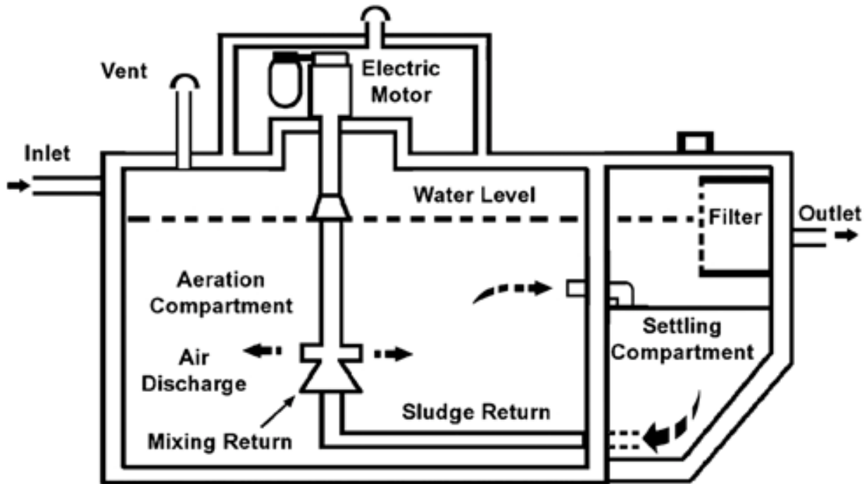
Figure 6.2.2.1.1: Conceptual Overview Aerobic Treatment Unit
