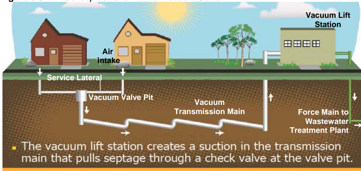
Figure 6.6.2.1: Conceptual Overview of Vacuum Sewer
